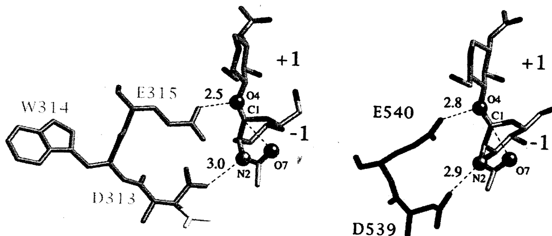
Figure 2. Conservation of chitinase A and chitobiase catalytic sites. The catalytic residues of chitinase A (left) and chitobiase (right) are shown and the overlap of the two enzymes (right). The -1 and +1 sugars are shown. Distances are given in Å. The complex of wild-type chitinase A with the substrate was modeled based on mutant complexes.
