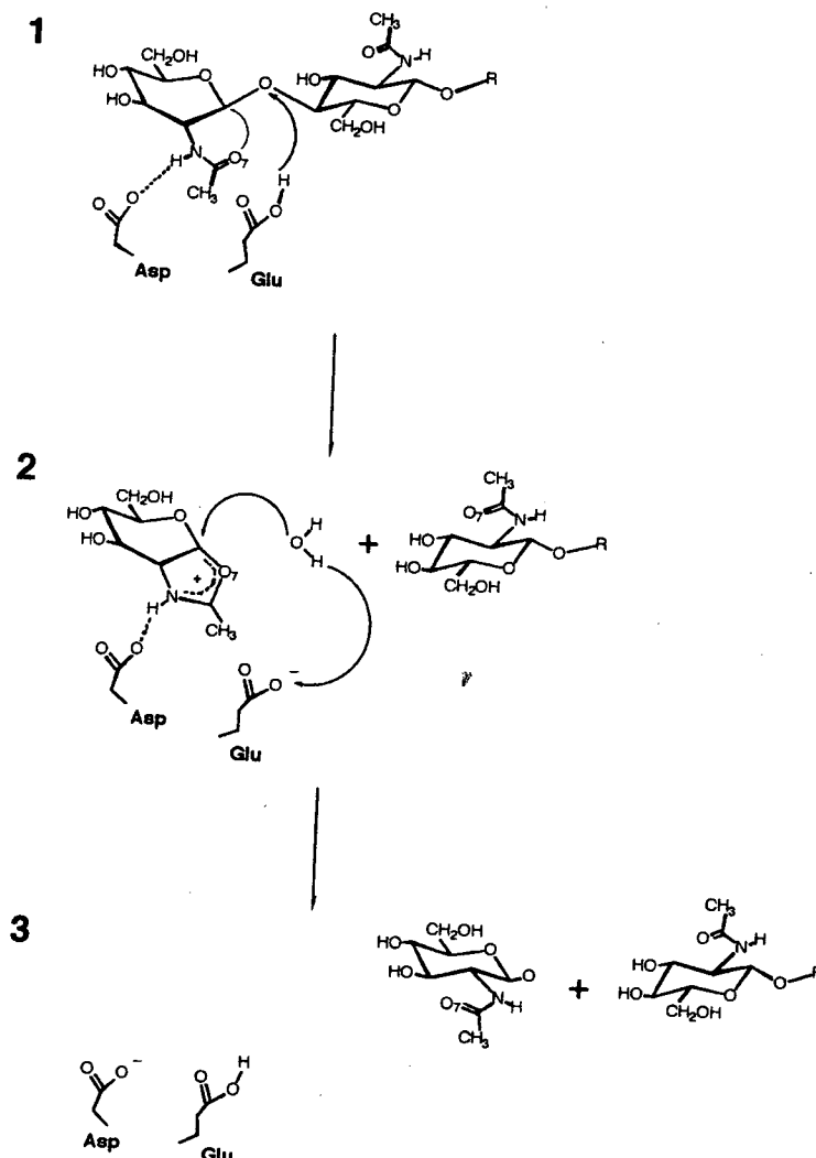
Figure 4. Model for the catalytic mechanism of chitinase A and chitobiase focusing on the catalytic Asp and Glu residues at the active site.
