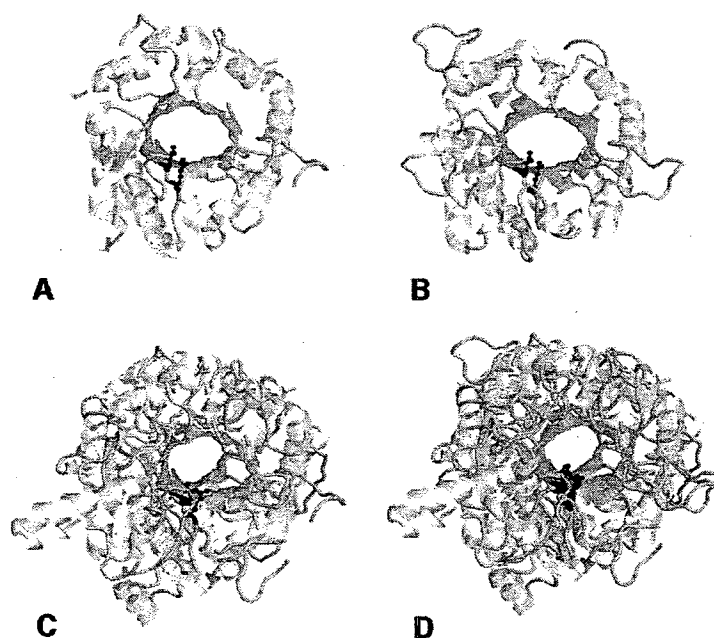
Figure 3. Structural comparison of the TIM-barrel domain of chitinase A (A), chitinase B (B), chitobiase (C) and superposition of all enzymes (D).
